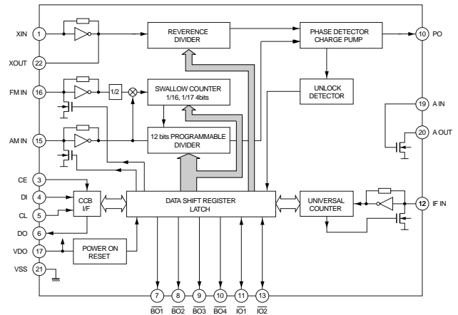
IC02 (LC72131)
